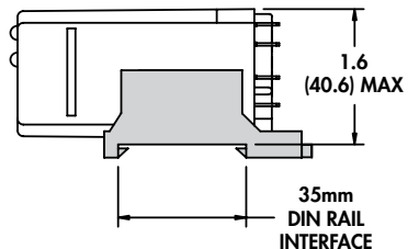
HORIZONTAL MOUNT (All Mating Relays)
