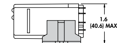
HORIZONTAL MOUNT (All Mating Relays)
